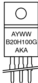
ISOLATED TO-220 CASE 221D STYLE 3
